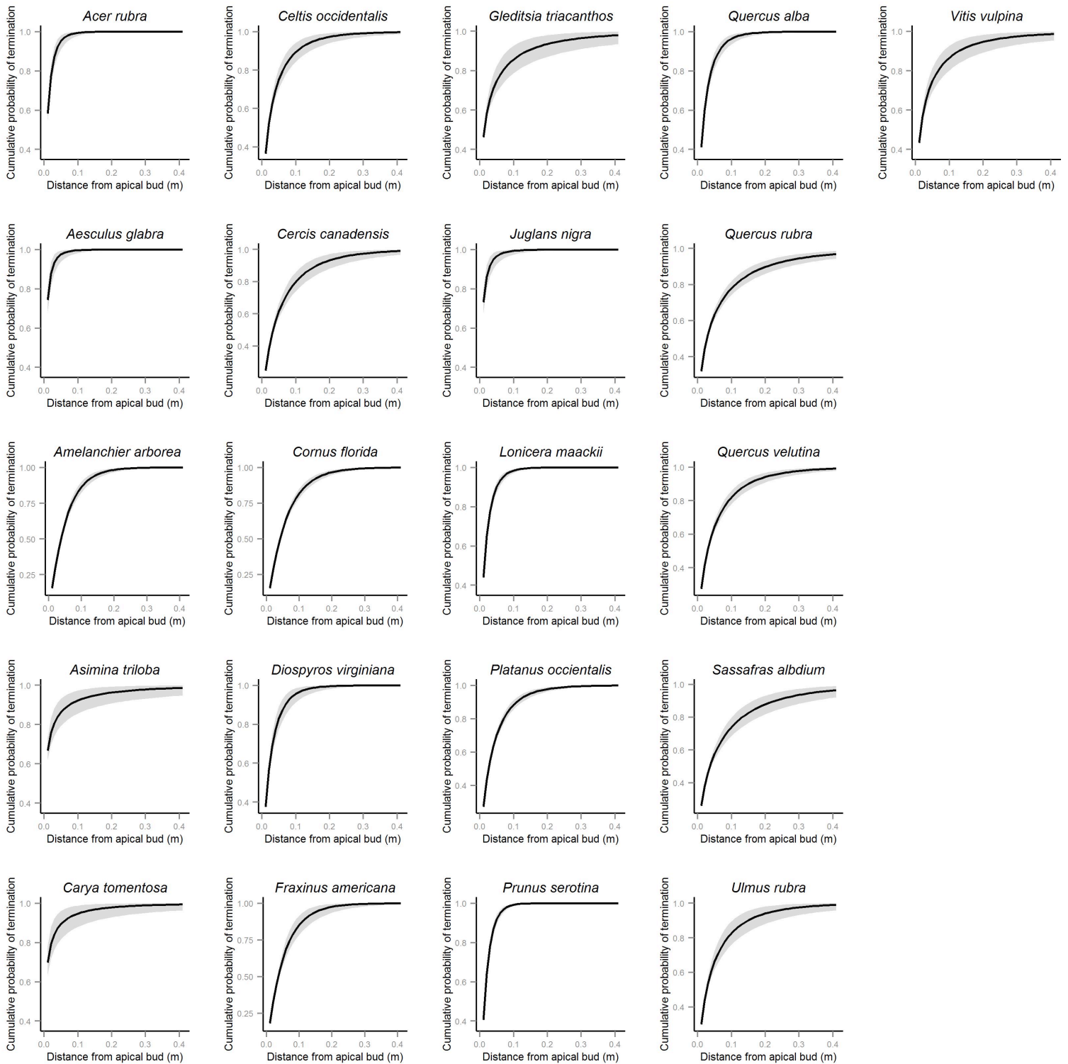
Figure S1: Vessel length distributions for 21 woody species based on the posterior means for the shape and scale parameters as estimated by model E (see methods) represented as the cumulative distribution function (CDF). The shaded areas represent 95% credible intervals.
